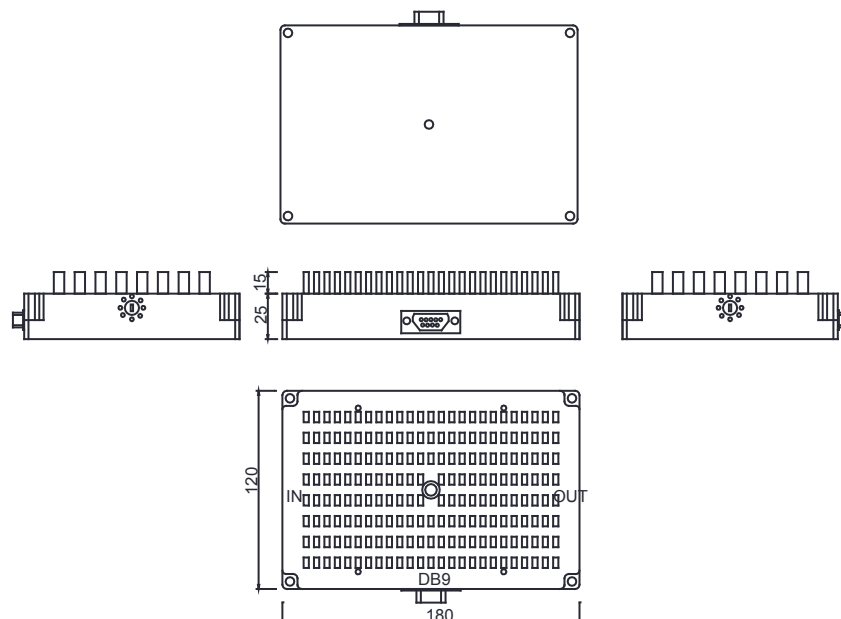
OUTLINE DRAWING(mm):
