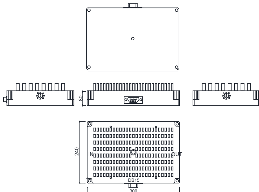
OUTLINE DRAWING(mm):
