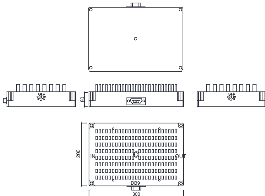
OUTLINE DRAWING(mm):
