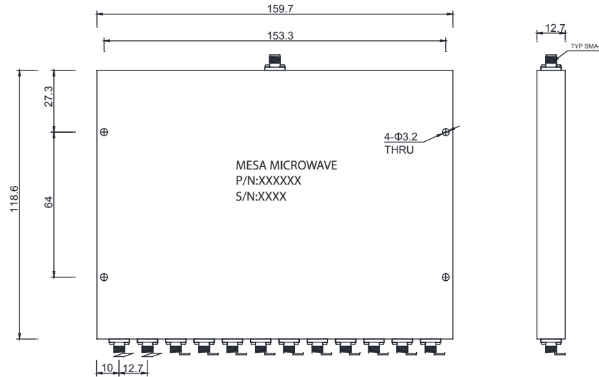
OUTLINE DRAWING(mm):
