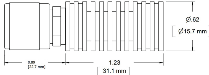
Dimensions IN[mm]
