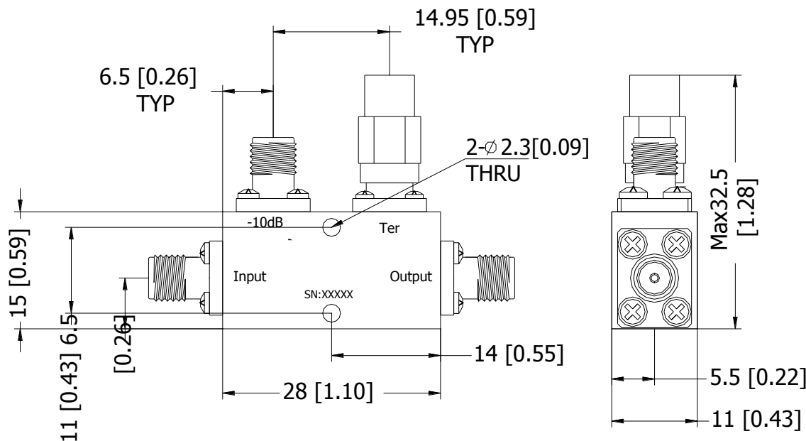
Dimensions mm[in]
